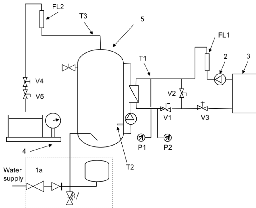
Figure F1.2 Apparatus example for unvented cylinder (EN12897) with external plate to plate
