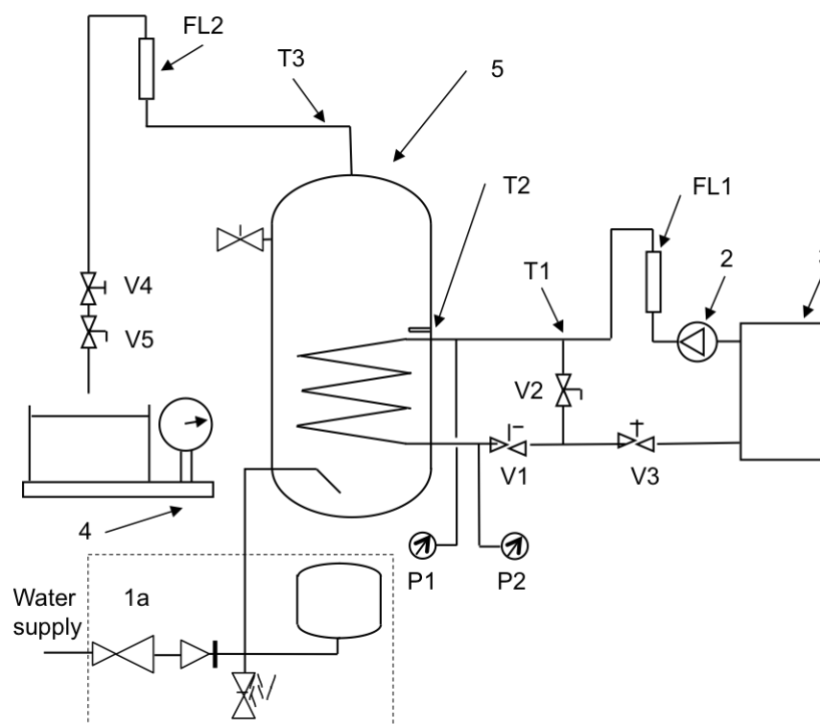
Figure F1.1 Apparatus example for unvented cylinder (EN12897) with internal coil type heat exchanger
